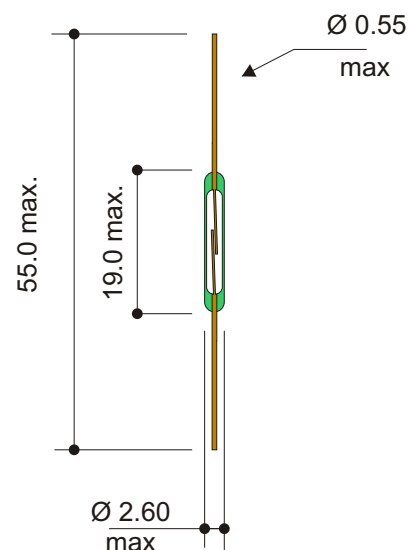
Dimensions expressed in mm
