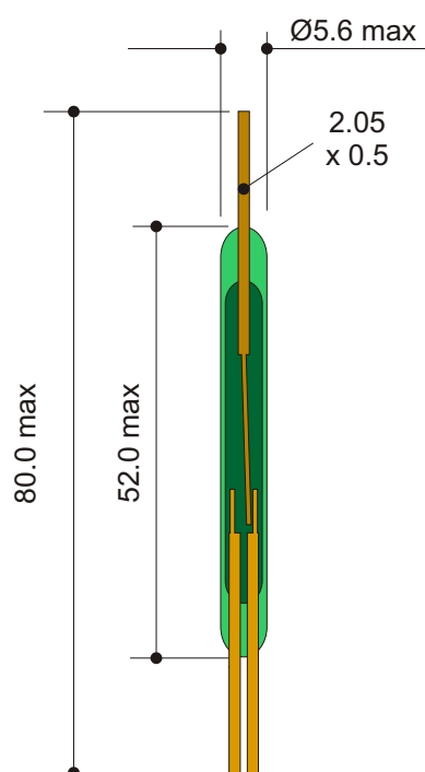
Dimensions expressed in mm
